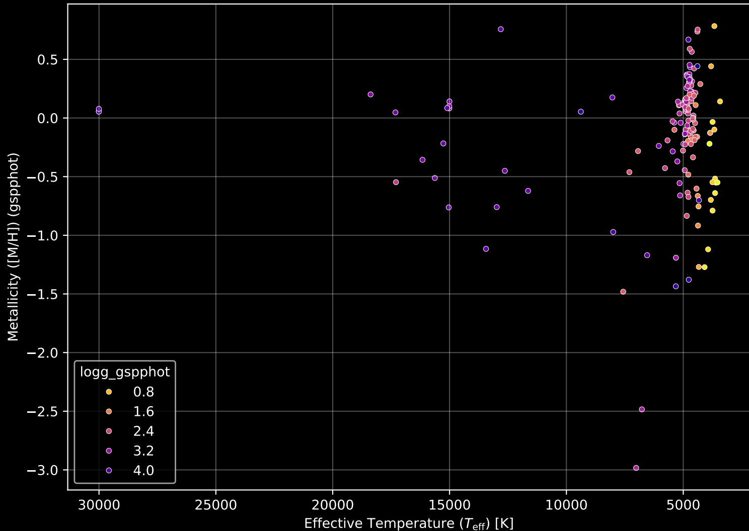
APOGEE DR17 Field: [020-02] Stellar Population Parameters (n= 158)
