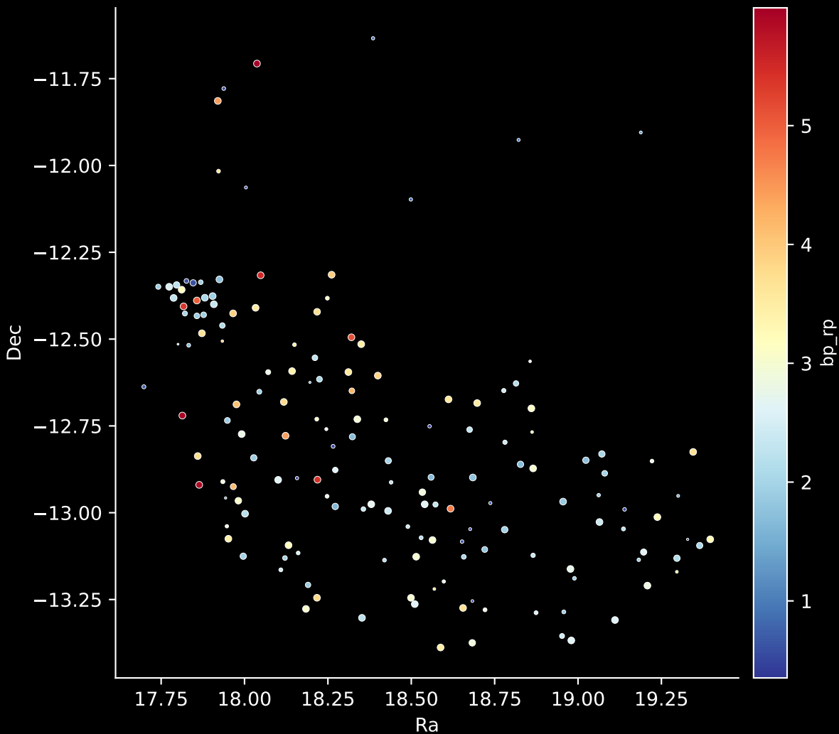
APOGEE DR17 Field: [020-02] Stars: 158
