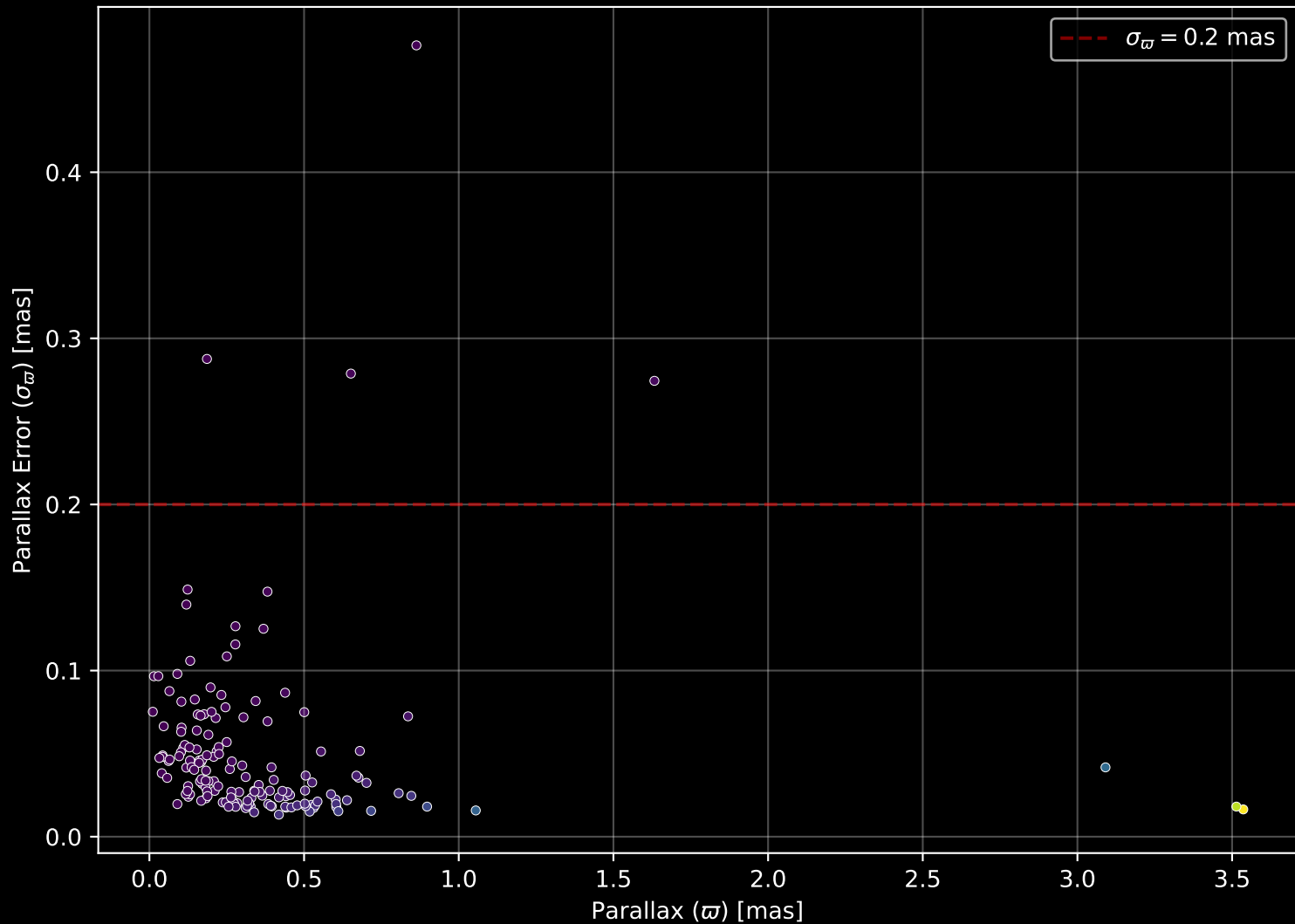
APOGEE DR17 Field: [020-02] Parallax Quality (n= 158)
