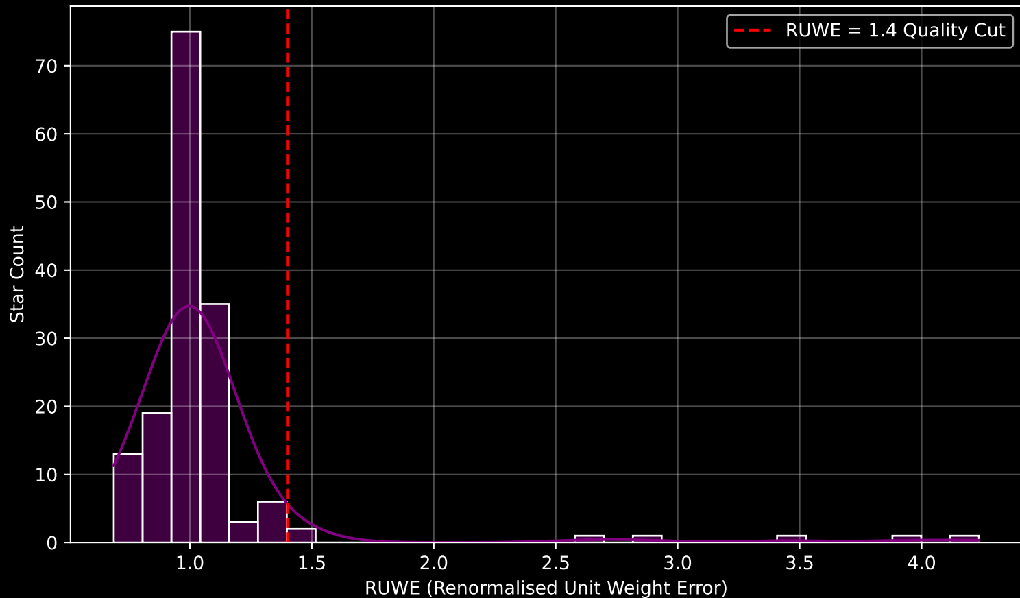
GAPOGEE DR17 Field [020-02] RUWE Distribution (n= 158)
