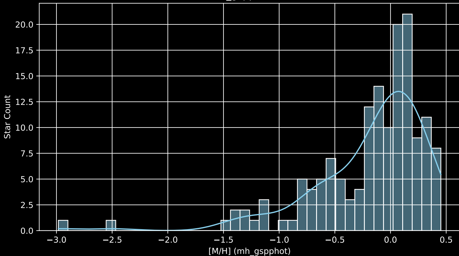
APOGEE DR17 Field: [020-02 [M/H] (mh_gspphot) (n= 151)
