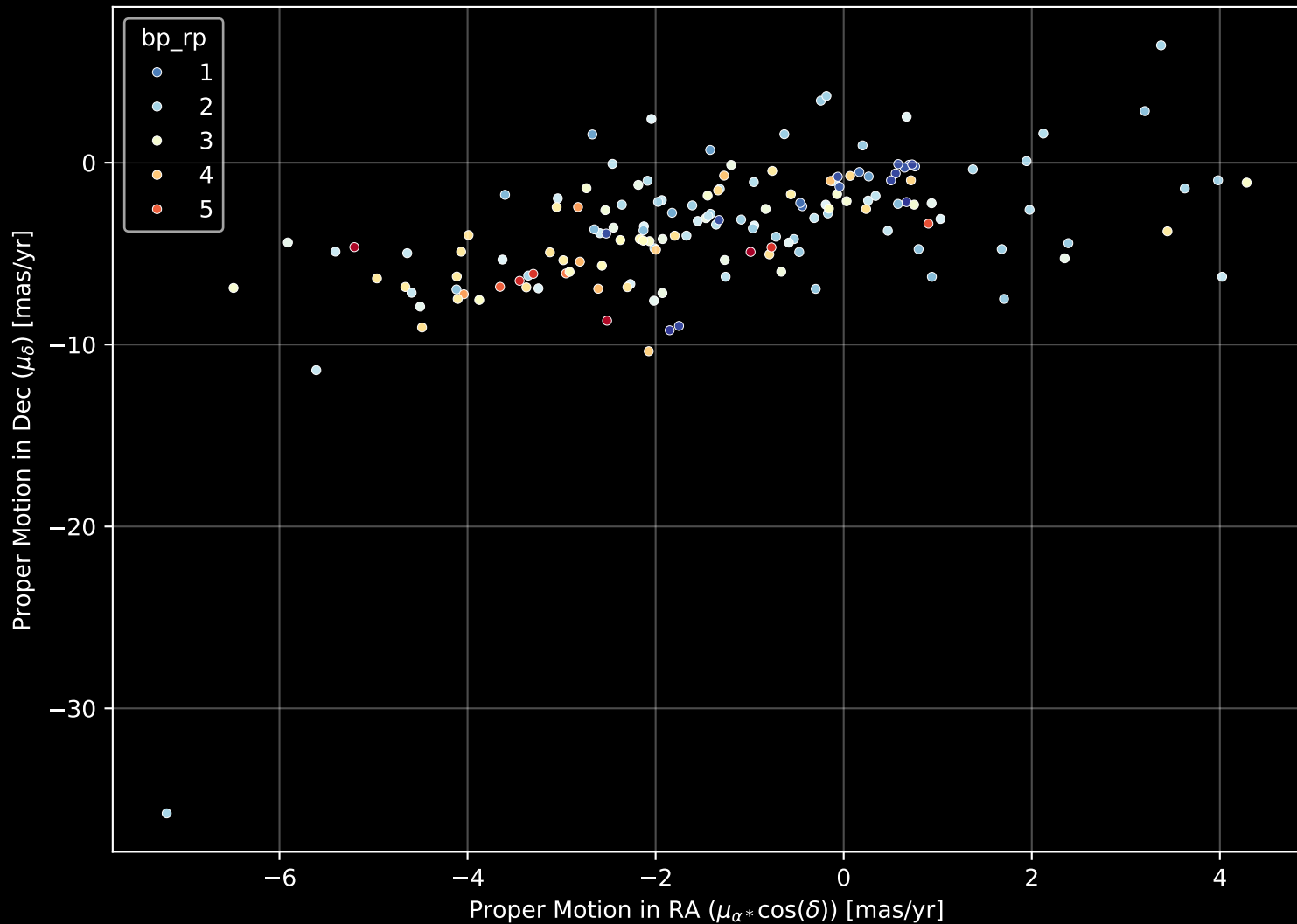
APOGEE DR17 Field: [020-02] Proper Motion Diagram (n= 158)
